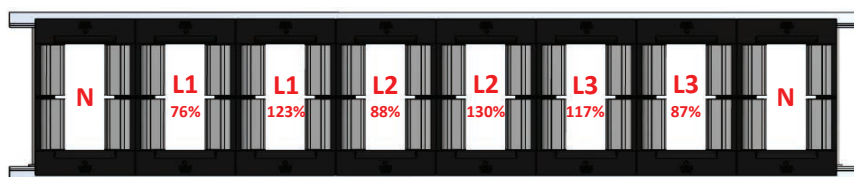
Non-Optimized Conductor Arrangement (Load current unbalanced)
