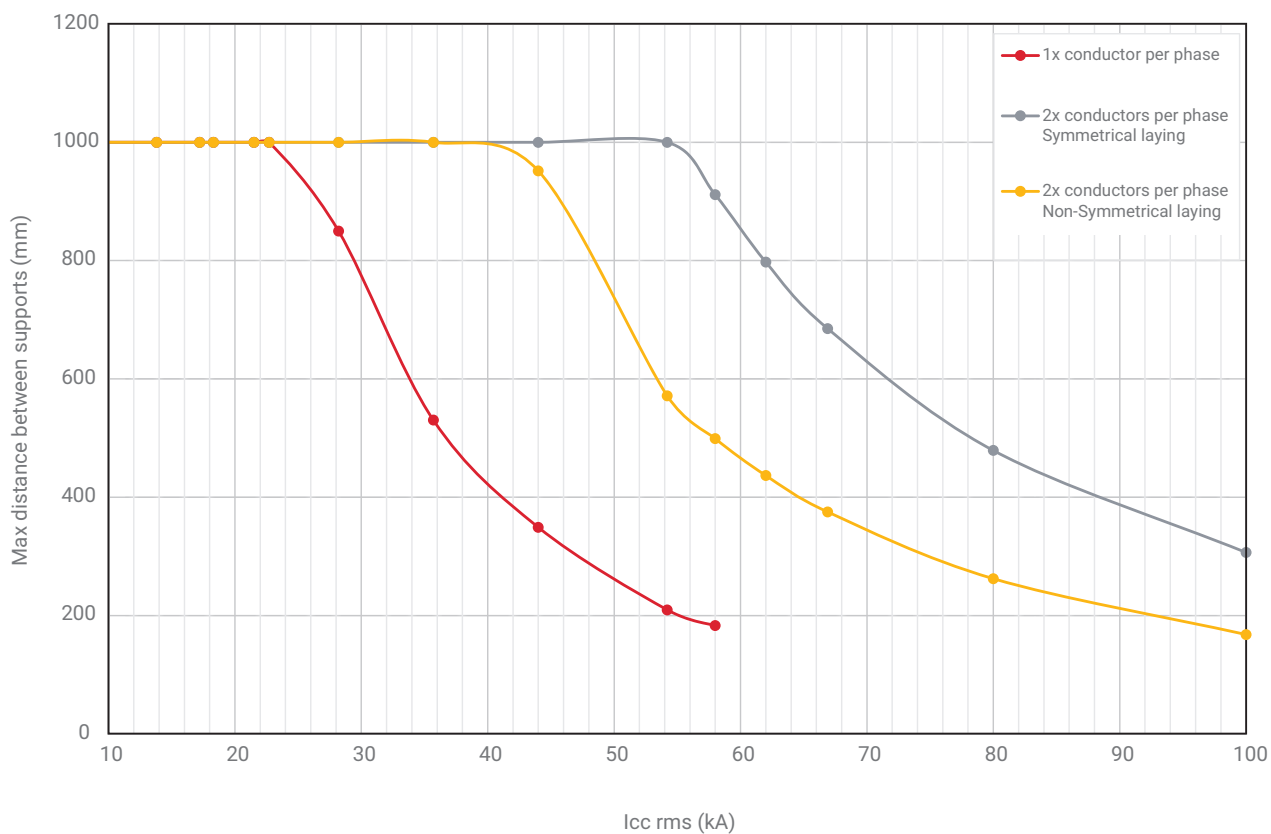
Maximum distance between axes of supports according to the I_{cc} rms values
